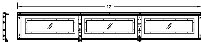
LOUVER - OPTIONAL IN BOTTOM SECTION
